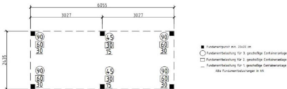
Fundamentplan - 20'
